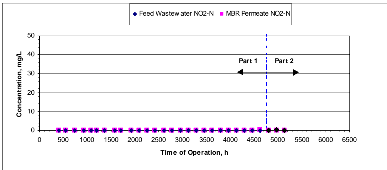
Figure 5-15: Inorganic Nitrogen Removal by the US Filter MBR
