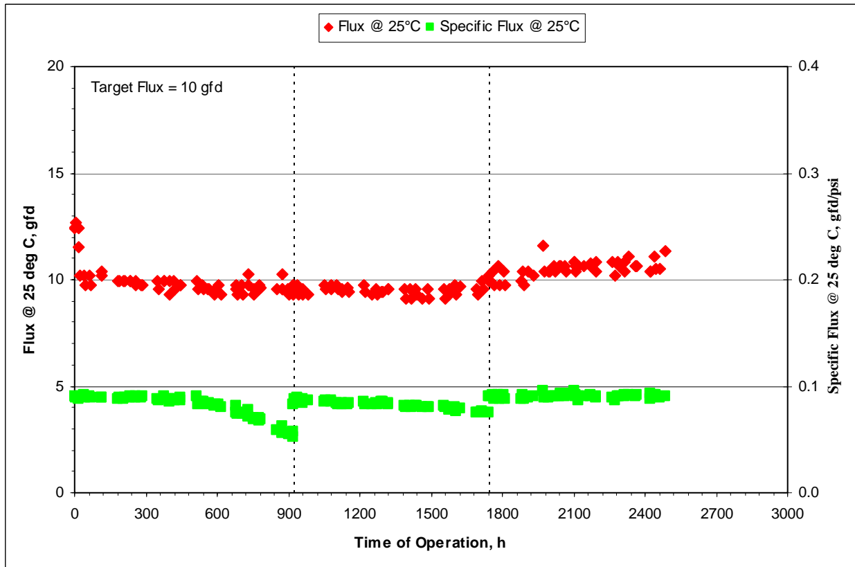
Figure 5-10: Hydraulics LFC3 RO Membrane Performance
