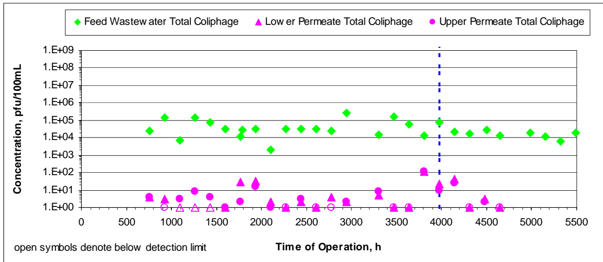
Figure 5-20: Coliform and Coliphage Removal by the Kubota MBR
