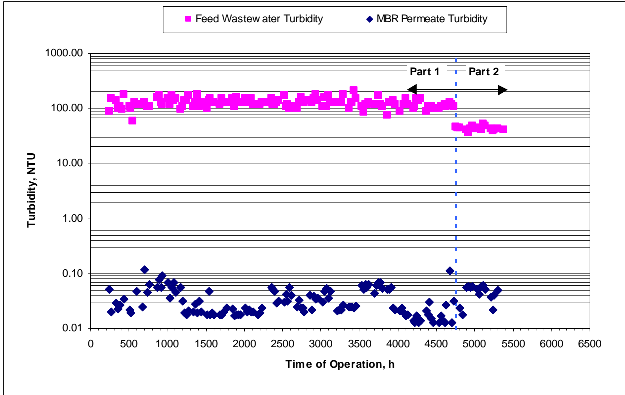
Figure 5-11: Turbidity Removal by the US Filter MBR
