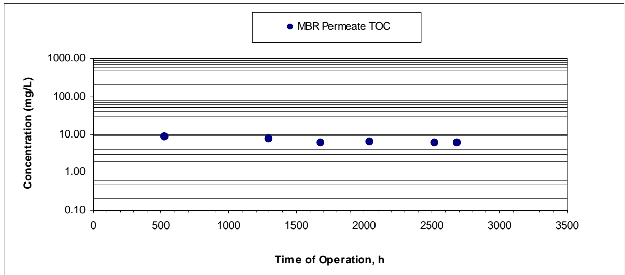
Figure 6-12: Organics Removal by the Zenon MBR
