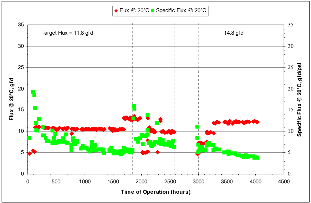
Figure 6-9: Membrane Performance of the Mitsubishi MBR
