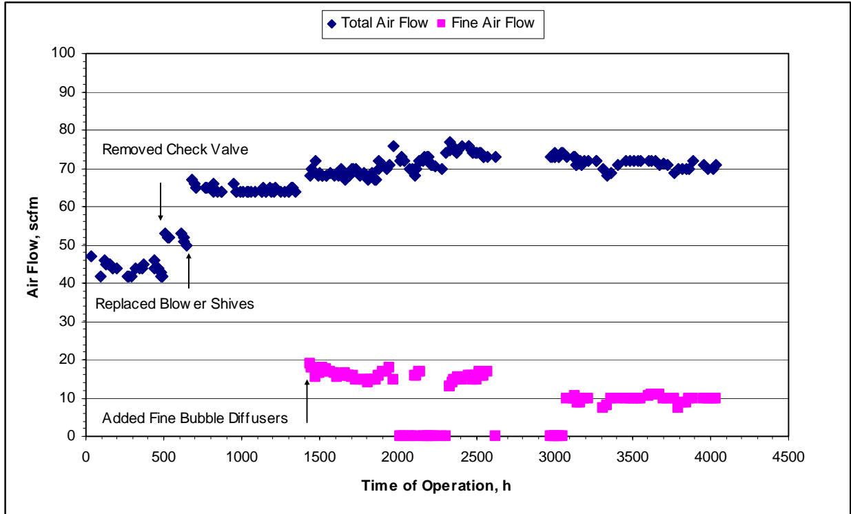
Figure 6-6: Air Flow to the Mitsubishi MBR
